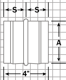
Male Coupling
